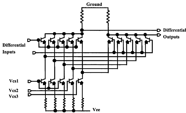
Fig. 4. CSH implementation of a basic CML gate. Five parallel (sub)transistor elements are used to maintain separate current paths.
