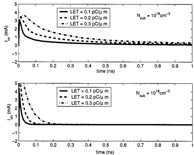
Fig. 8. SEE-induced collector and emitter currents for \text{LET} = 0.1, 0.2 and 0.3 \text{ pC}/\mu\text{m} . N_{sub} = 10^{18}/\text{cm}^3 .
