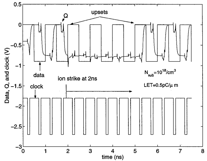
Fig. 5. Simulated SEE response of the D-flip-flop for N_{\text{sub}} = 10^{18}/\text{cm}^3 and \text{LET} = 0.5 \text{ pC}/\mu\text{m} .
