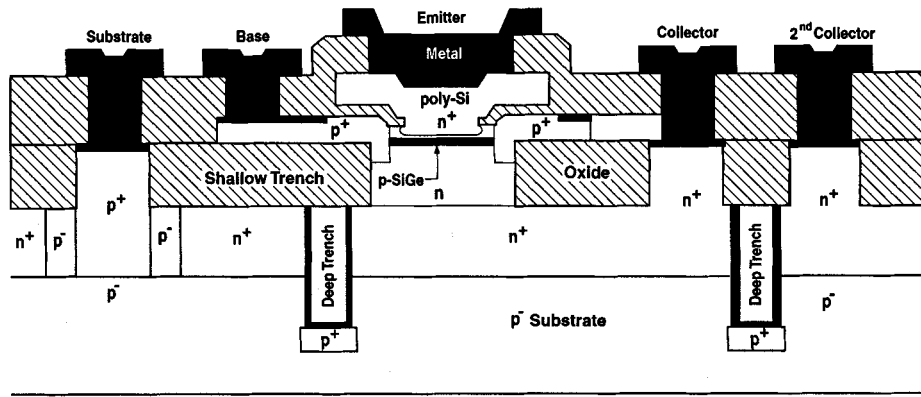
Fig. 1. The schematic cross section of the SiGe HBT used in simulation.
