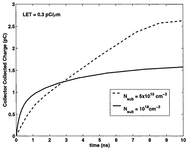
Fig. 13. Collected charge as a function of time for N_{sub} = 5 \times 10^{15} and 10^{18}/\text{cm}^3 . LET = 0.3 pC/ \mu\text{m} . Charge column length is 10 \mu\text{m} .
