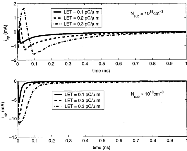
Fig. 9. SEE-induced base and substrate currents for LET = 0.1, 0.2 and 0.3 pC/\mu m . N_{sub} = 10^{18}/cm^3 .
