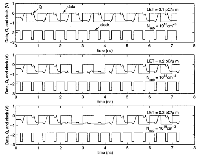
Fig. 7. Simulated SEE response of the D-flip-flop for \text{LET} = 0.1, 0.2, and 0.3 \text{ pC}/\mu\text{m} . N_{sub} = 10^{18}/\text{cm}^3 .
