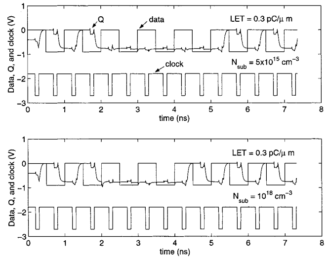
Fig. 10. Simulated SEE response of the D-flip-flop for N_{sub} = 5 \times 10^{15}/cm^3 and N_{sub} = 10^{18}/cm^3 . LET = 0.3 pC/\mu m .
