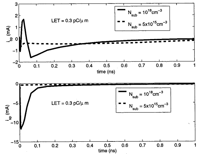
Fig. 12. SEE-induced transient base and substrate currents for N_{sub} = 5 \times 10^{15} and 10^{18}/cm^3 . LET = 0.3 pC/\mu m .
